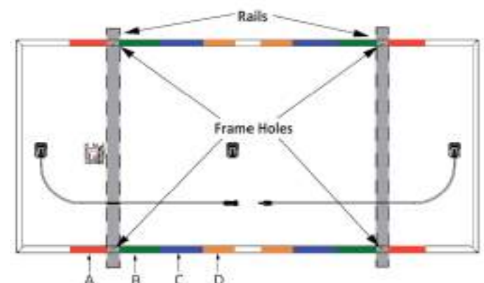
Figure 4: Mounting Zone Locations for Performance modules
